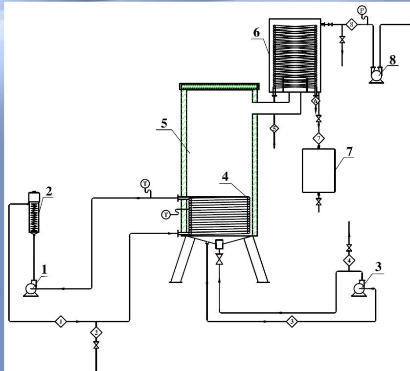
Machine for herb extraction and vacuum evaporation
