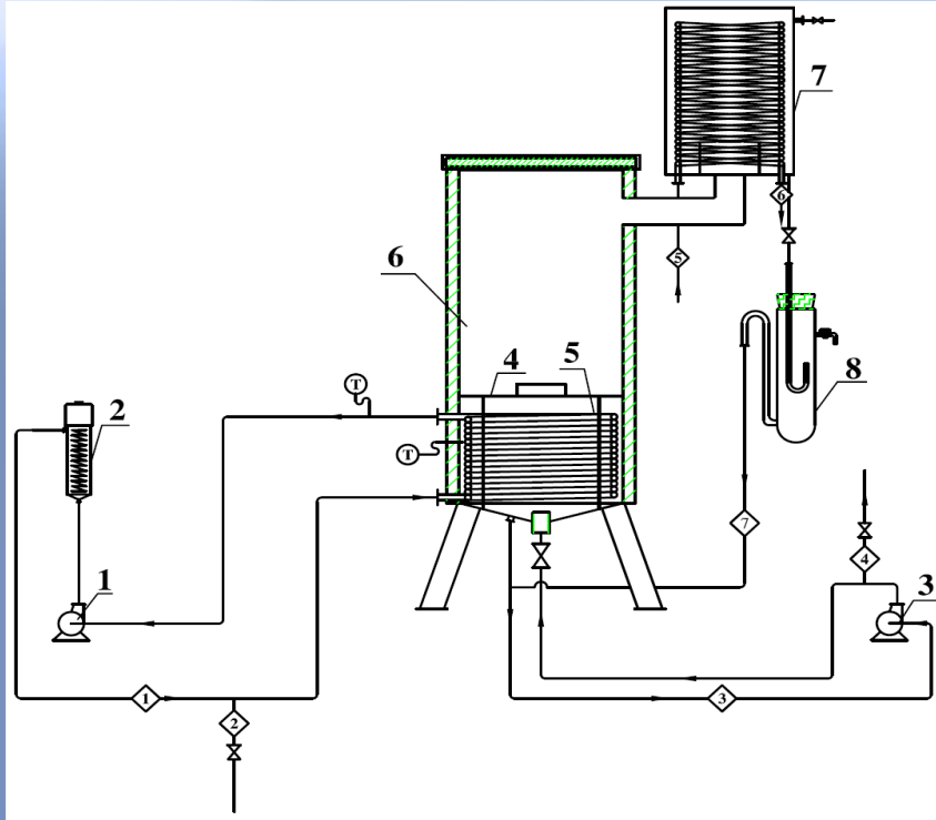
Machine for steam distillation
